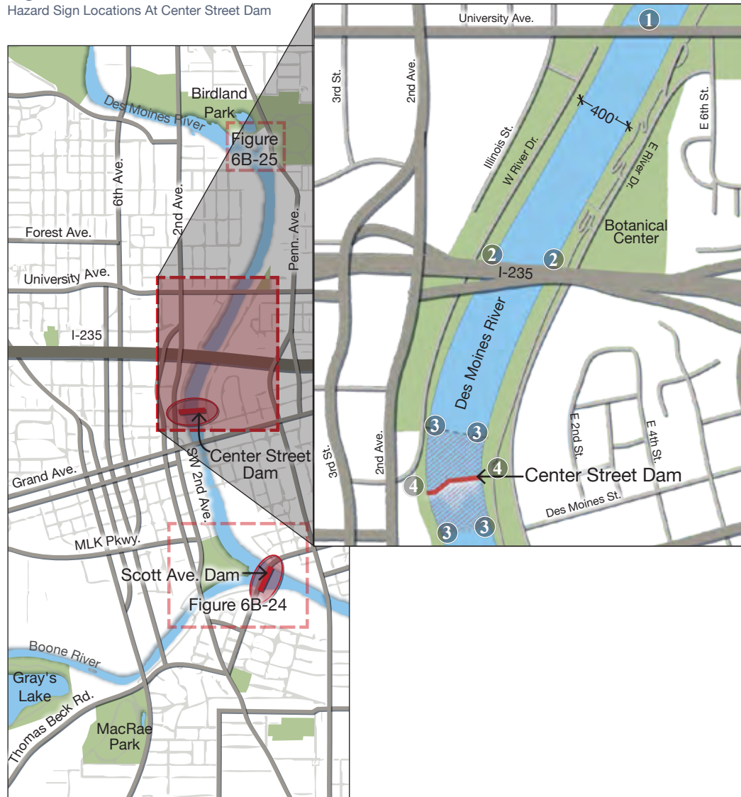
Figure 6B-26. Hazard Sign Locations At Center Street Dam
